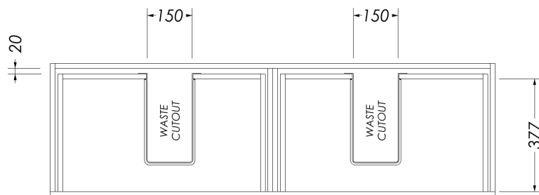
TOP & BOTTOM DRAWER CROSS SECTION
